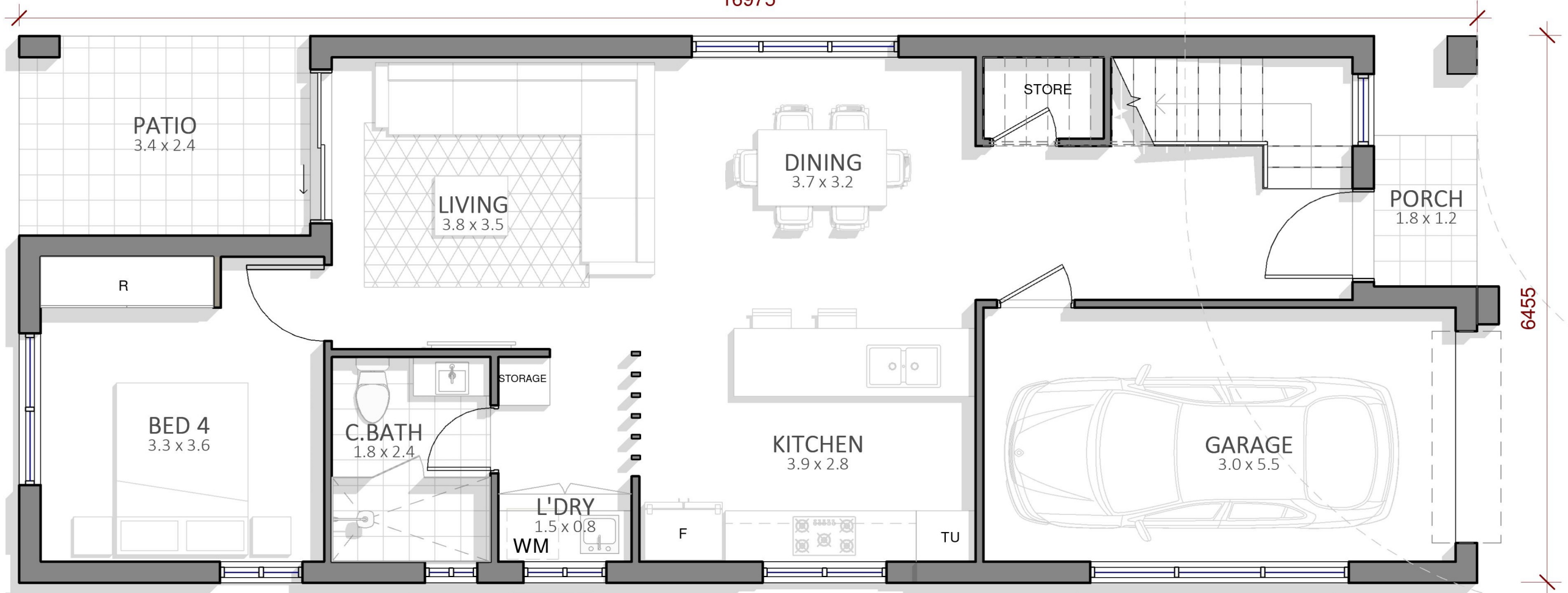
Ground Floor
