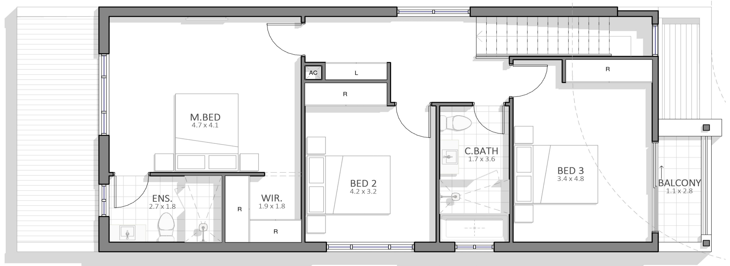
First Floor
