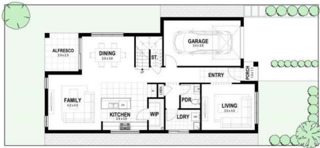
GROUND FLOOR 1:100
