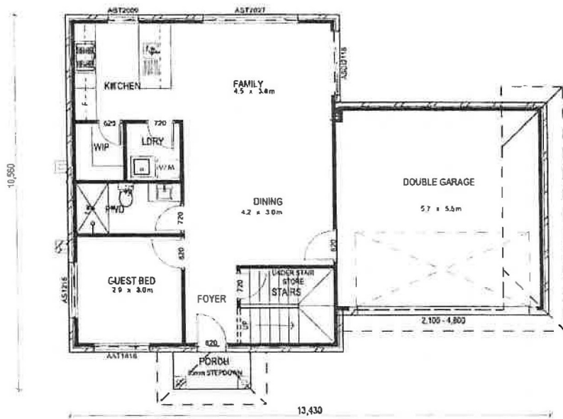
GROUND FLOOR PLAN 1:100 01
