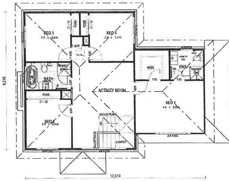
FIRST FLOOR PLAN 1:100 03
