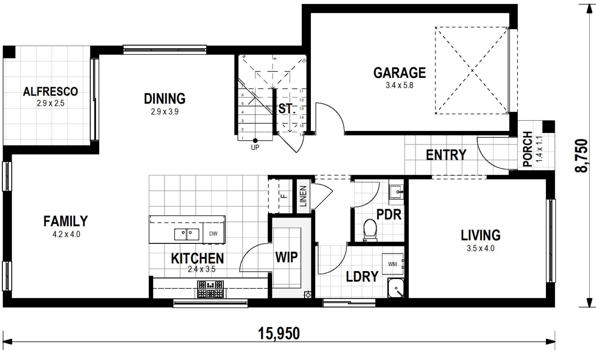
GROUND FLOOR 1:100
