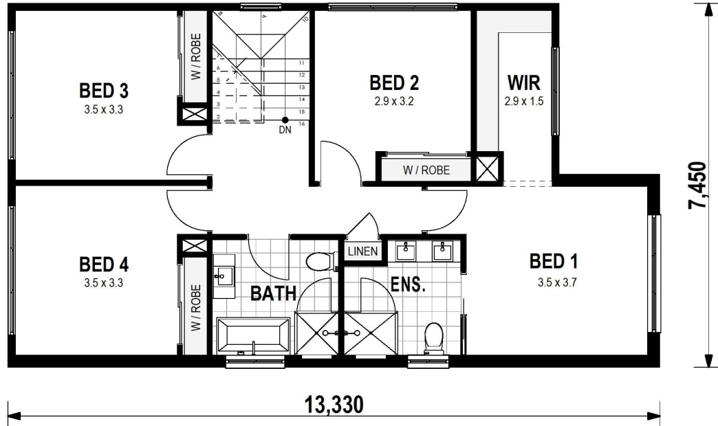
FIRST FLOOR 1:100
