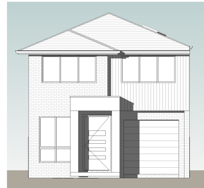
CONCEPTUAL ELEVATION
