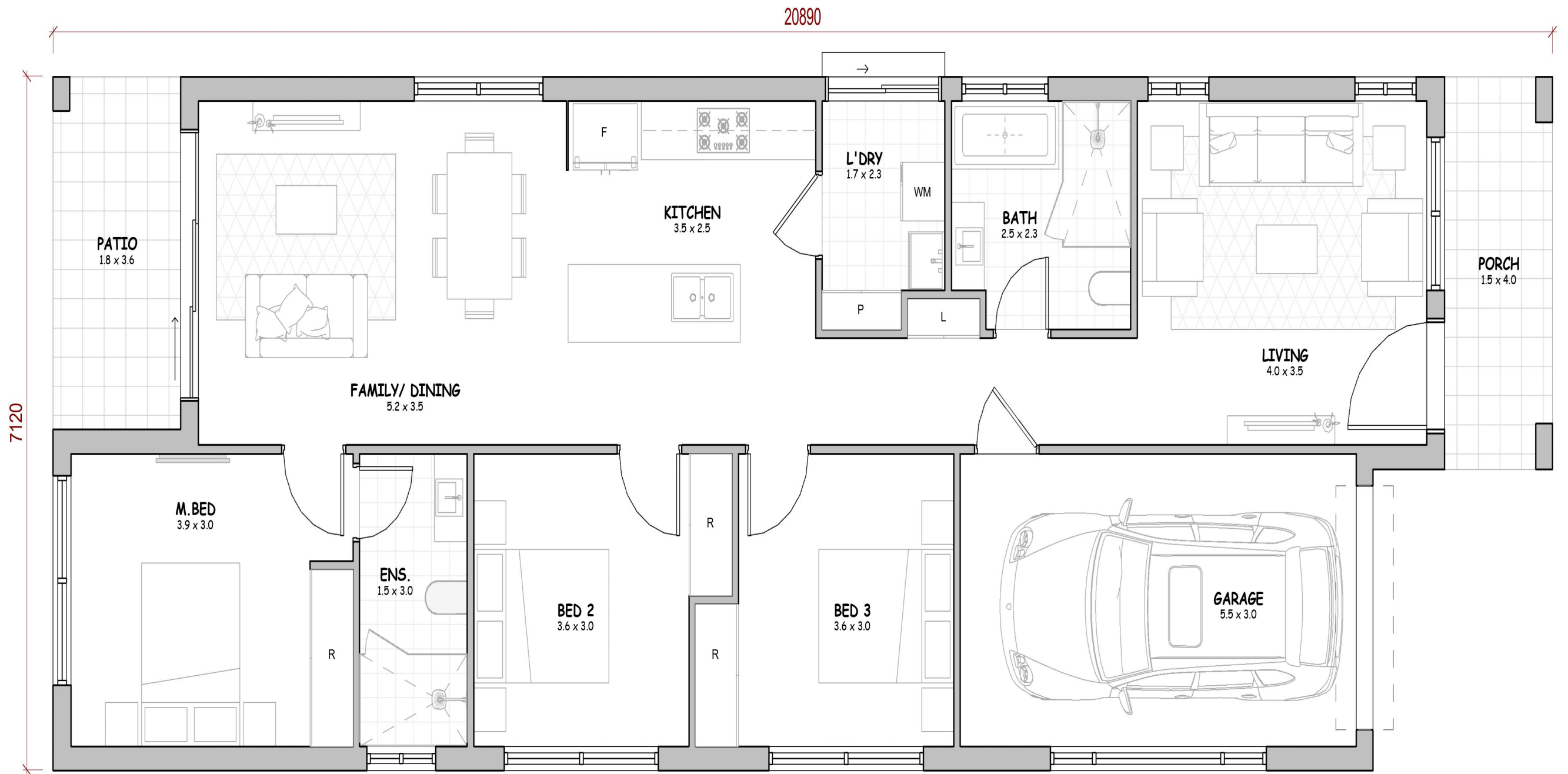
FLOOR PLAN
