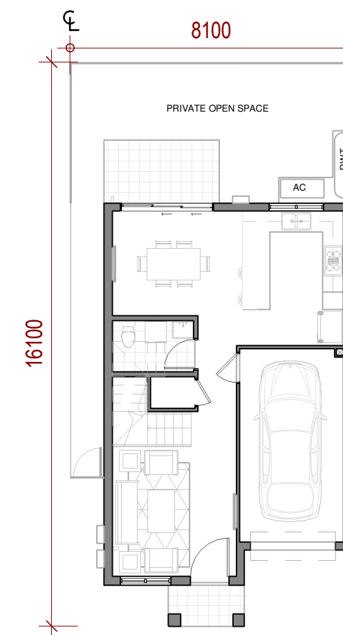
LOT PLAN
