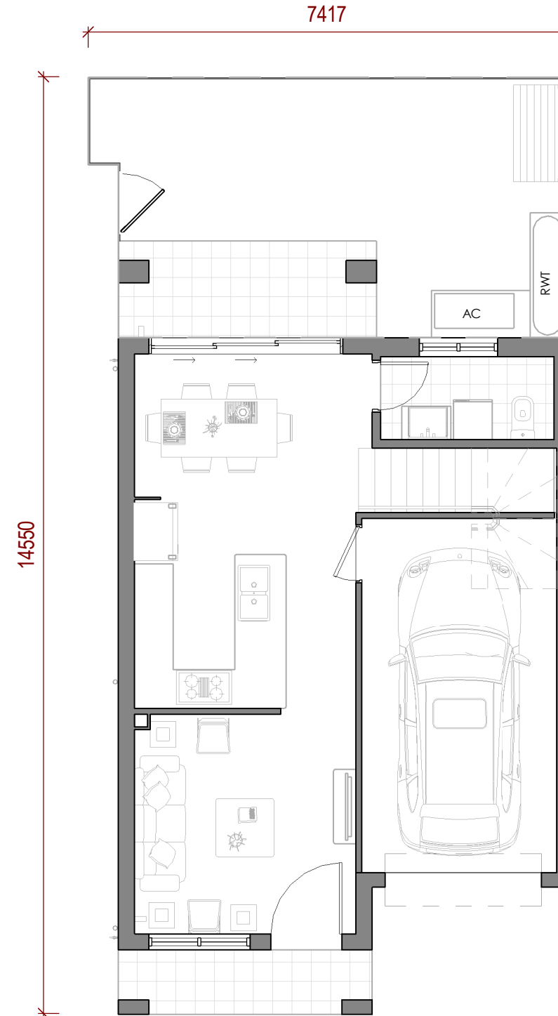
LOT PLAN
