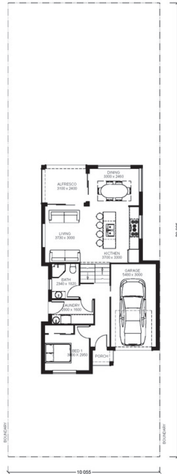
Ground floor
