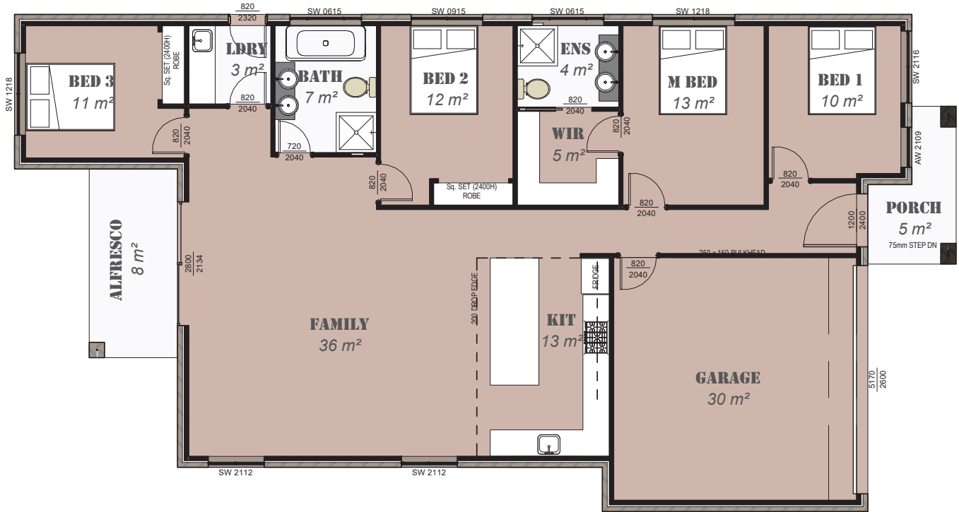
FLOOR PLAN HOUSE LENGTH = 20.5 m HOUSE WIDTH = 11.25 m
