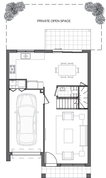
PROPERTY PLAN
