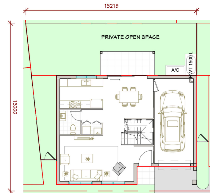
PROPERTY PLAN
