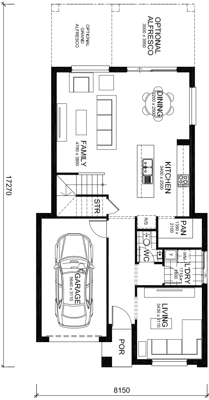
GROUND FLOOR
