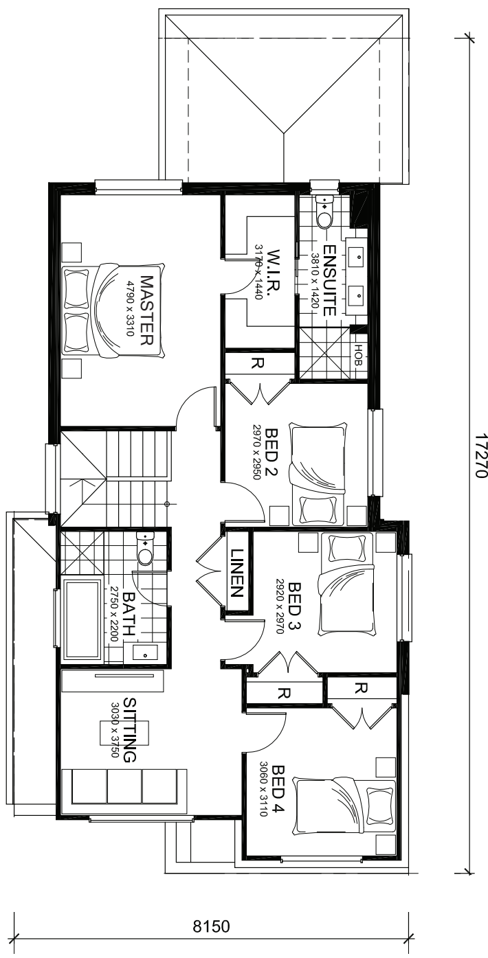
FIRST FLOOR
