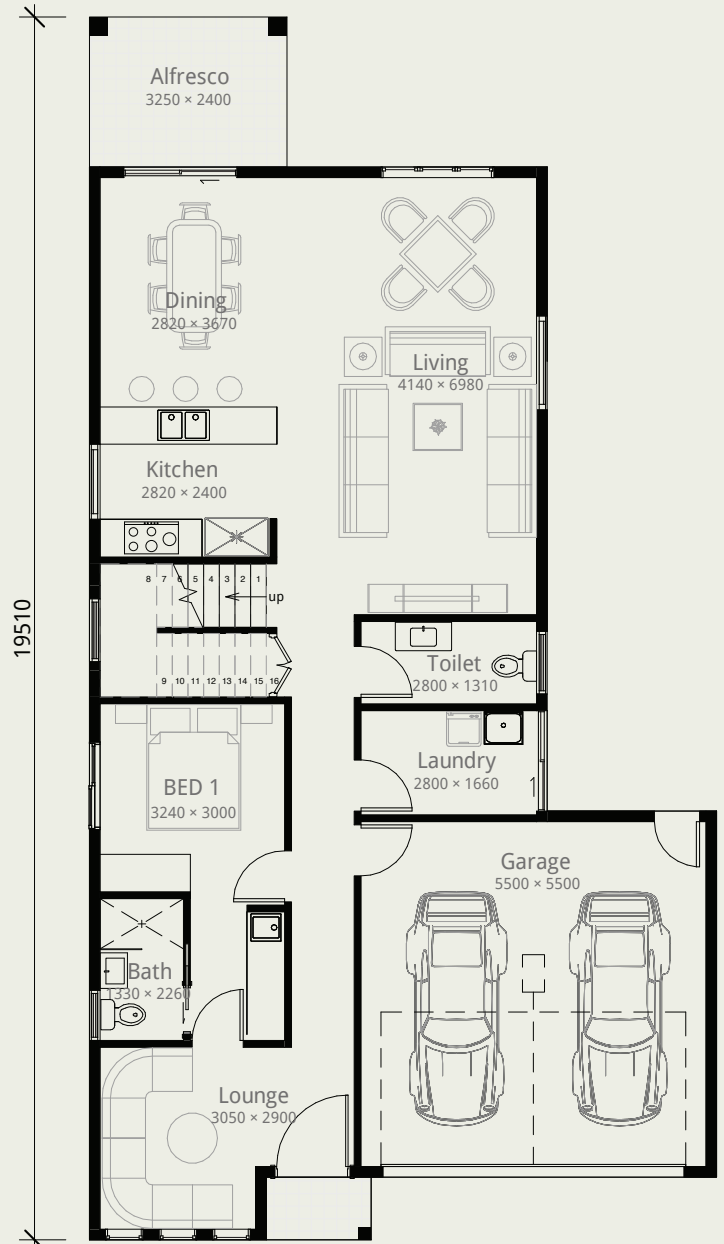
10000 Ground Floor Plan
