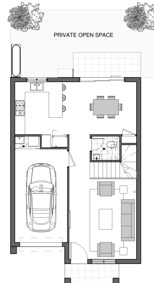
PROPERTY PLAN
