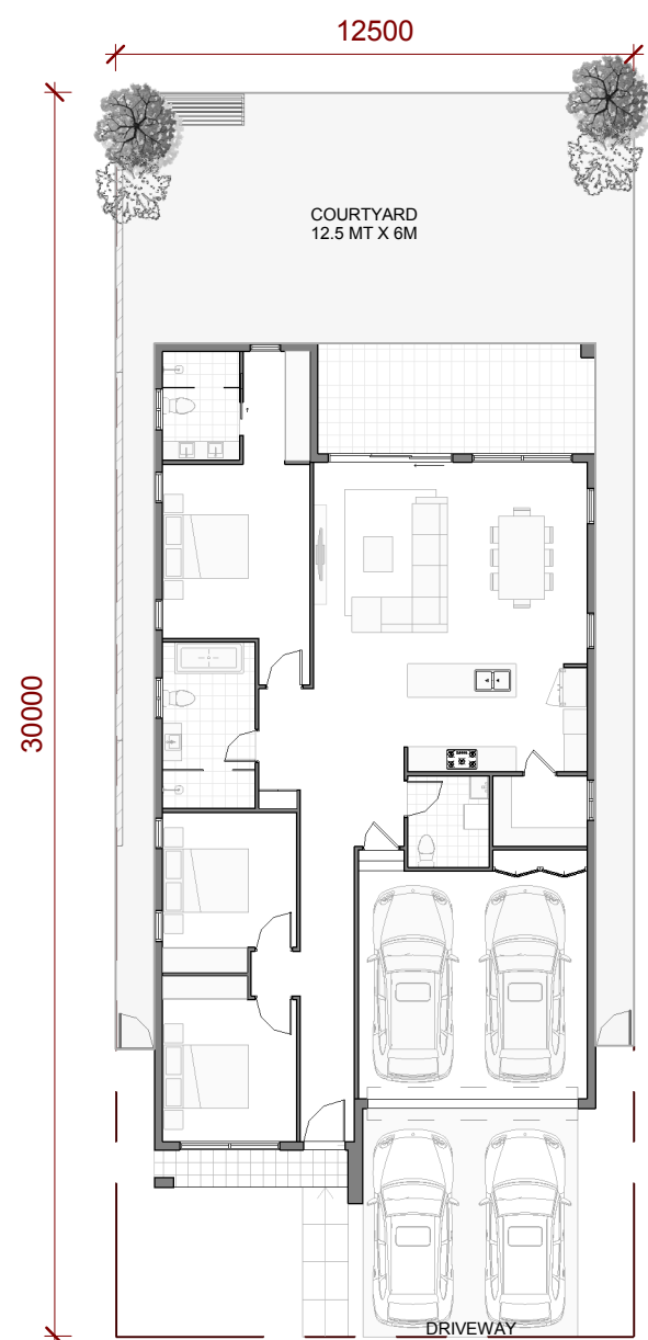
LOT PLAN
