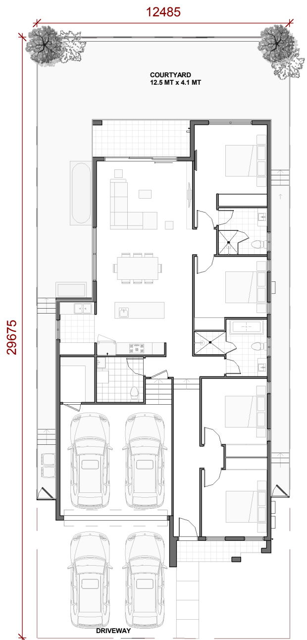
LOT PLAN
